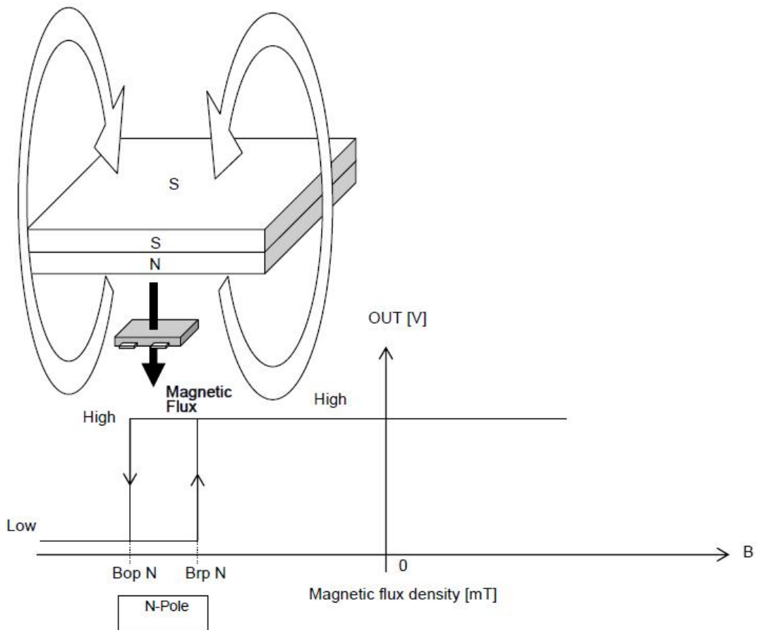
Fig 4, Magnetic Operation Characteristic of AS1511
