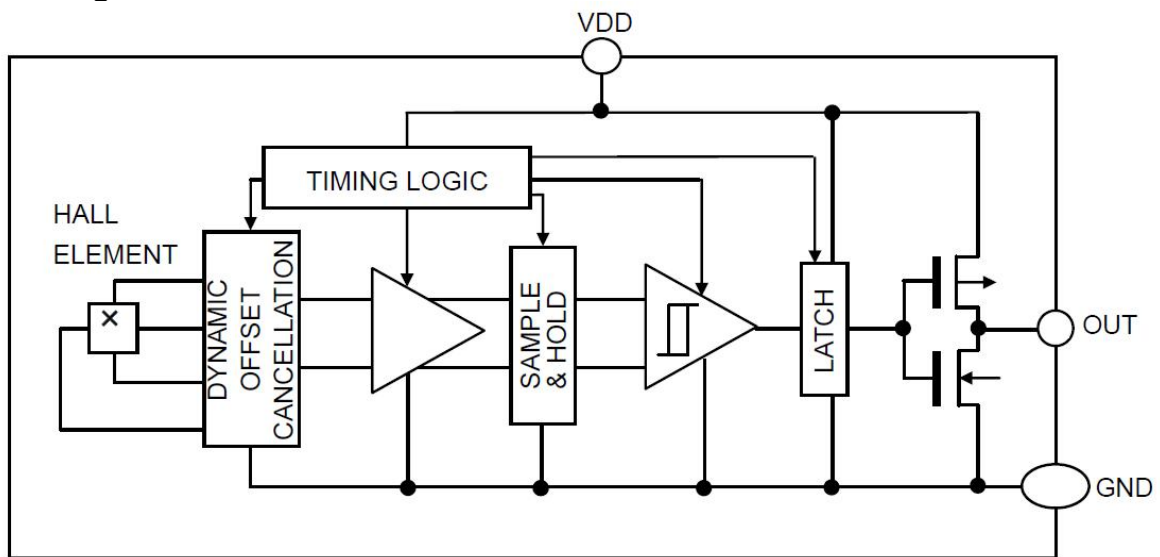
Figure 3, Block Diagram of AS1511
